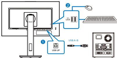
USB hub
